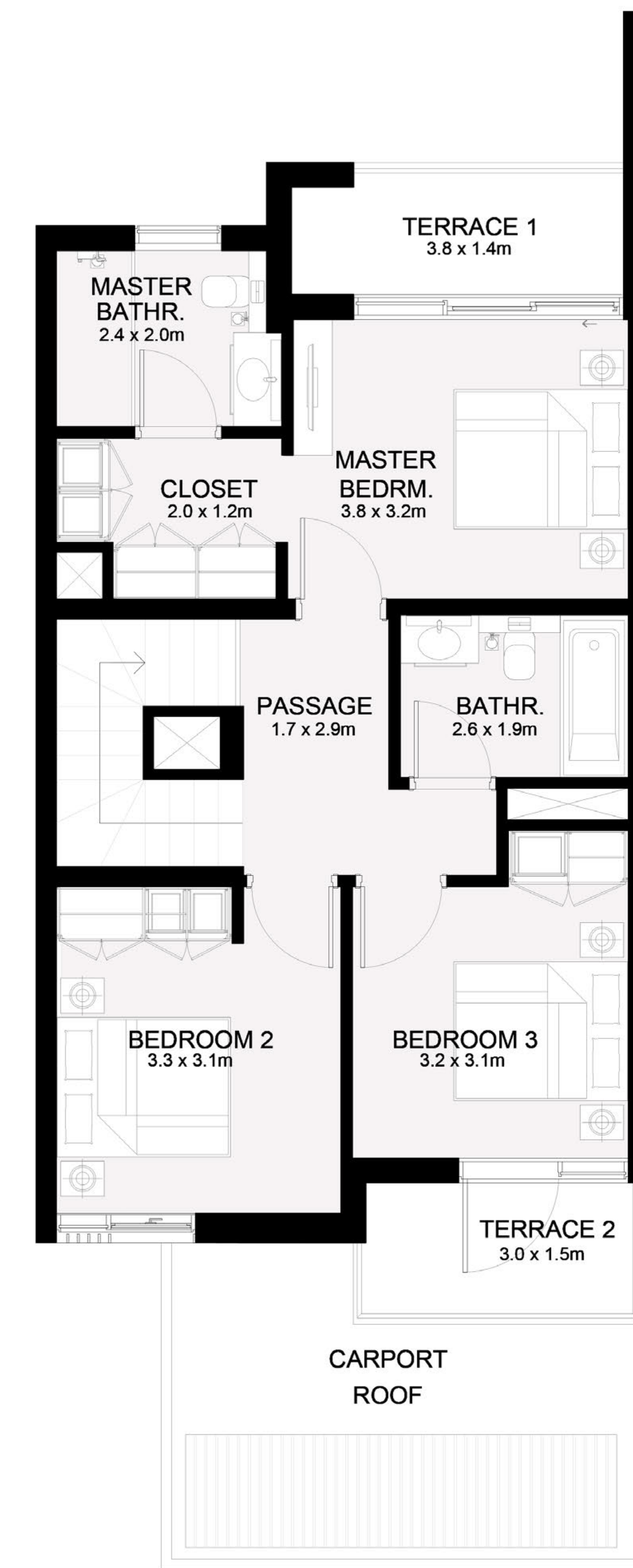
FIRST FLOOR
