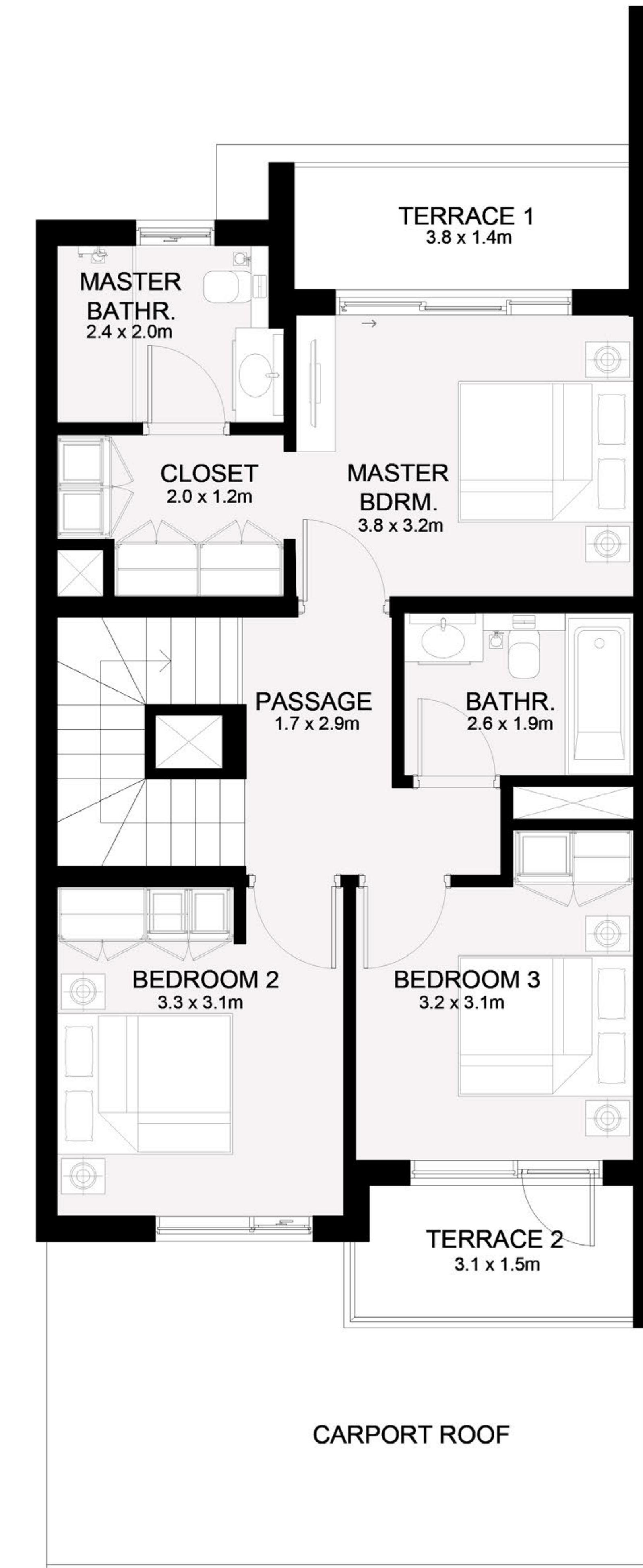
FIRST FLOOR
