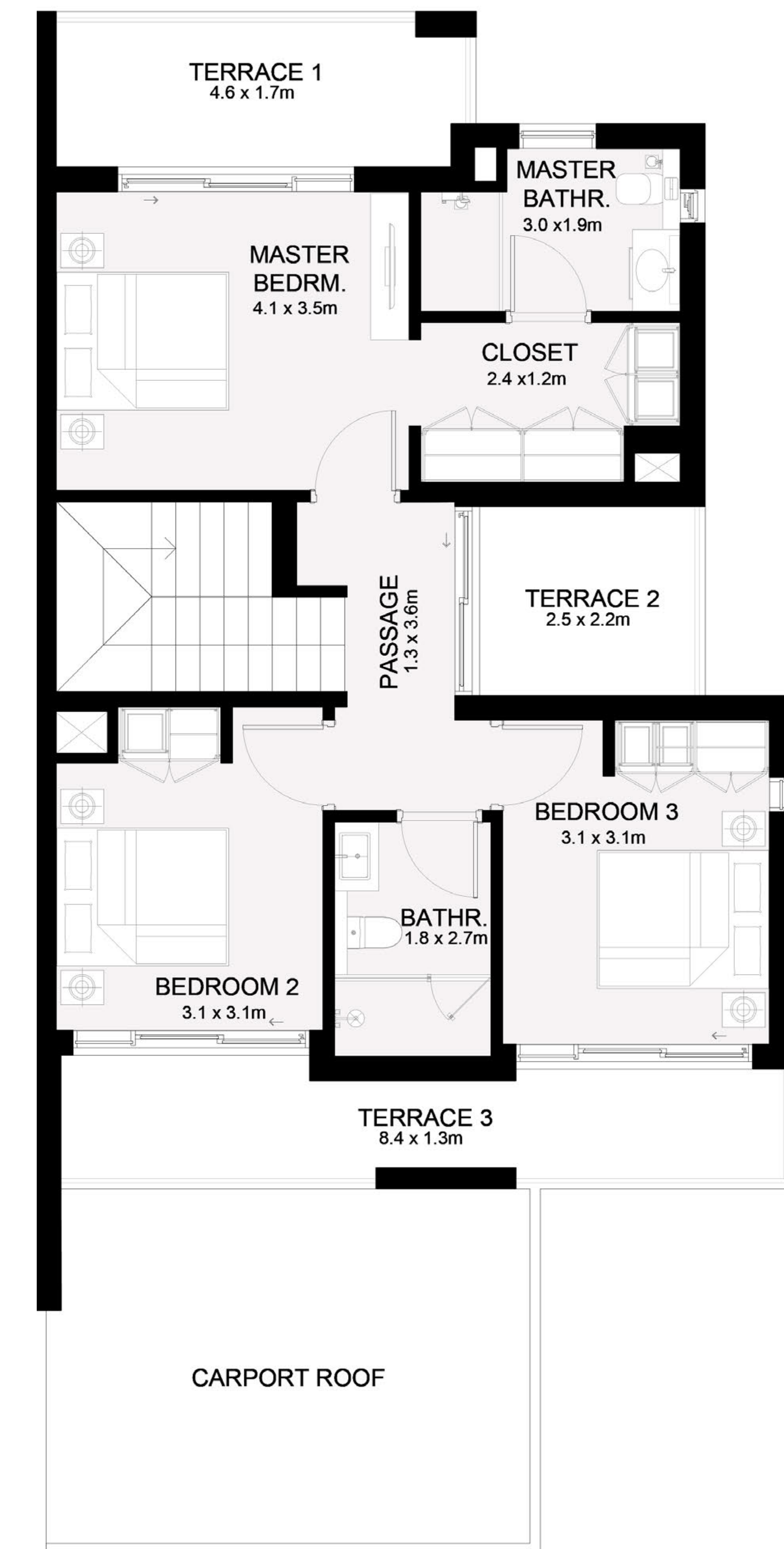
FIRST FLOOR
